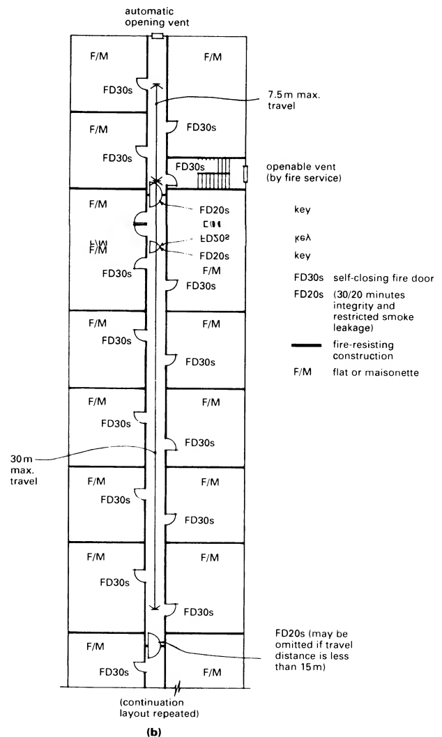
② Typical arrangements for flats or maisonettes with more than one common stair according to the Building Regulations for England and Wales: (a) corridor access, (b) corridor access with dead ends
